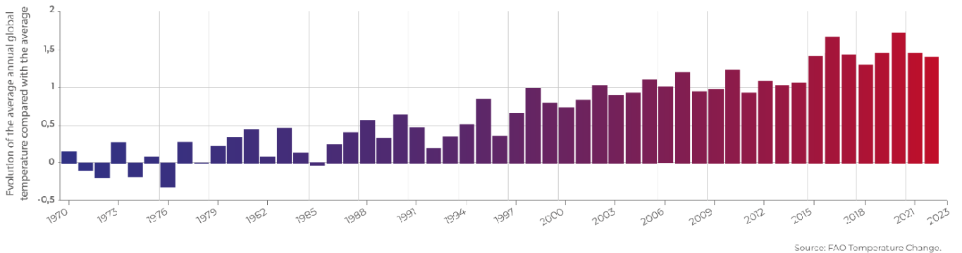
Figure 1 – Increase in annual global average temperature from 1970 to 2023 in comparison to the average from 1951 to 1980
