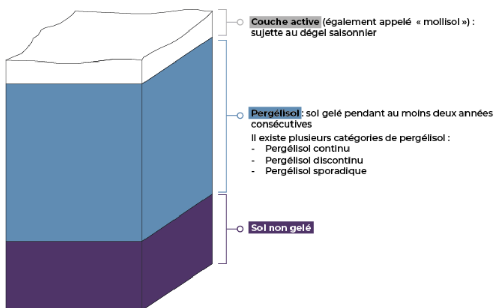
Figure 2 – Structure du pergélisol
